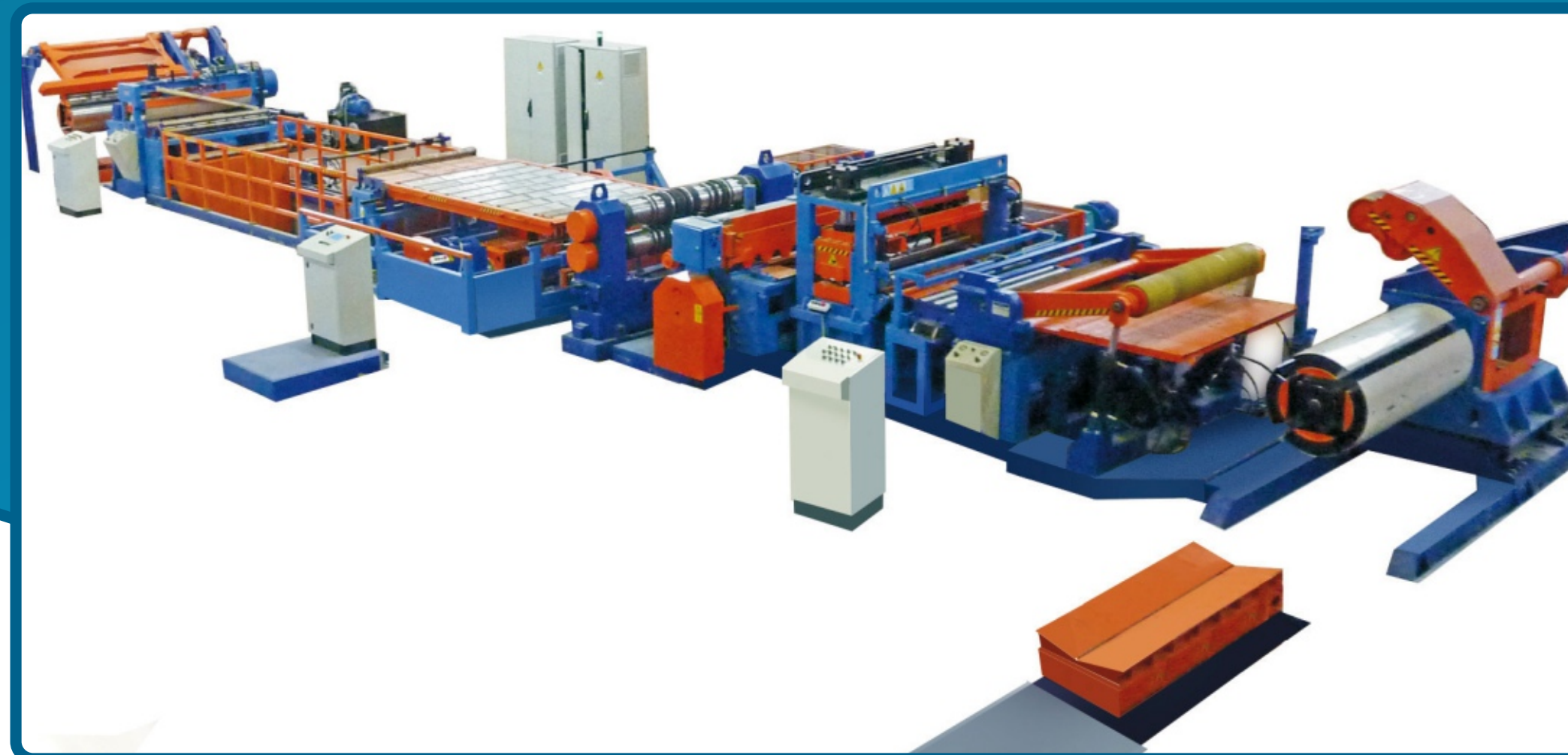
Automatic Line of Length Cutting of Coiled Metal
